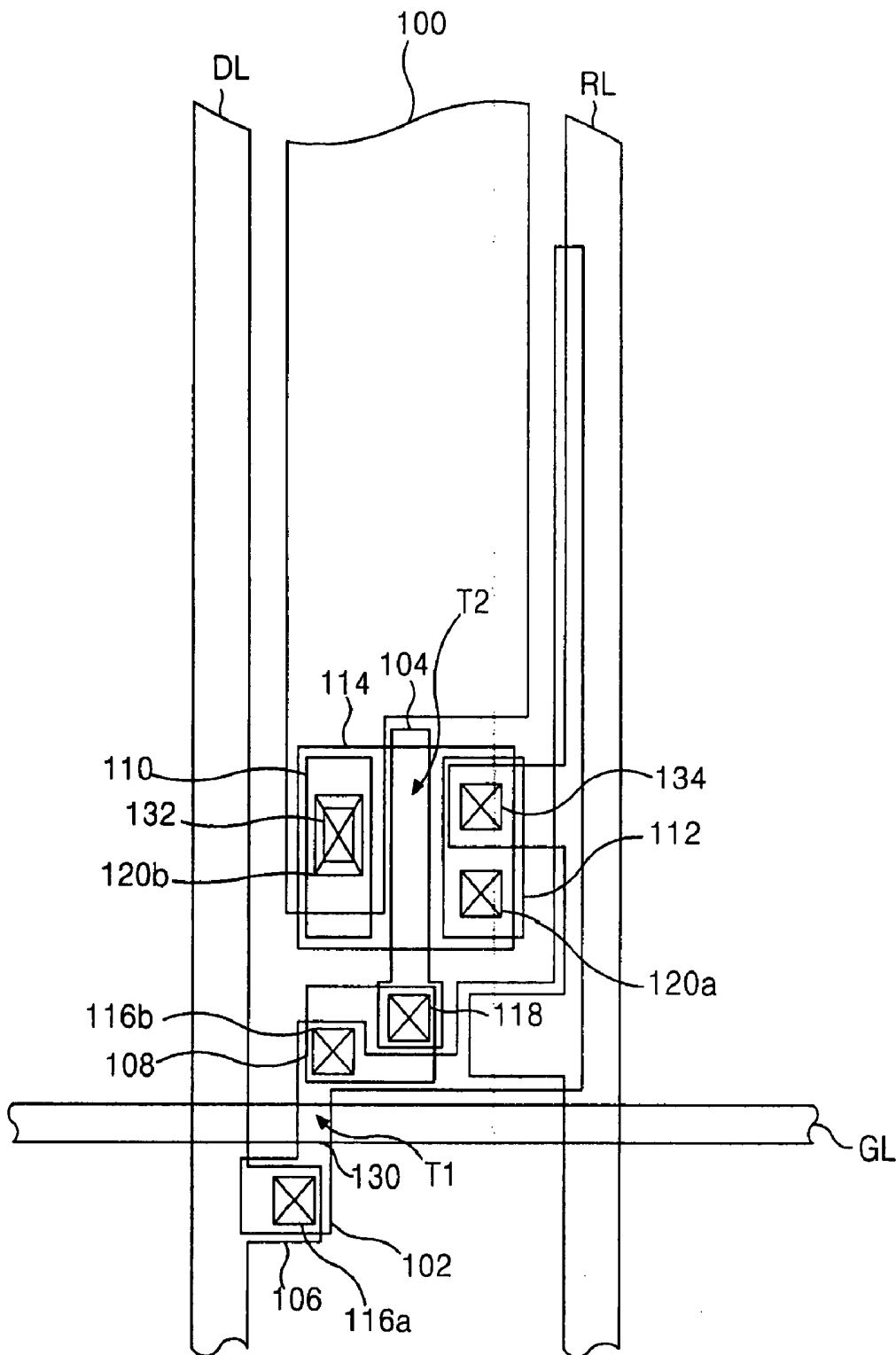
FIG. 3 RELATED ART
